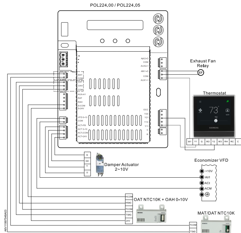
Fig. 2: Single Enthalpy Switchover + VFD + Thermostat + Exhaust Fan + Damper Actuator + OAT & MAT Sensors + OAH Sensor
